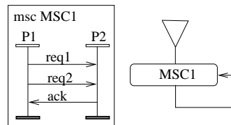
Fig. 4. An MSC Specification with no process divergence
