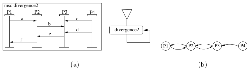
Fig. 6. (a) MSC example divergence2 ; (b) its Coordination graph
