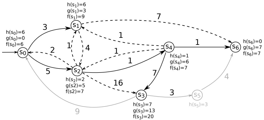
Figure 11: The explored part of G (2), see the example in Section 4.6. The faintly gray vertices and edges have not yet been explored by A^* . The solid edges indicate the current search tree of A^* , whereas dashed line edges are the sidetrack edges.
