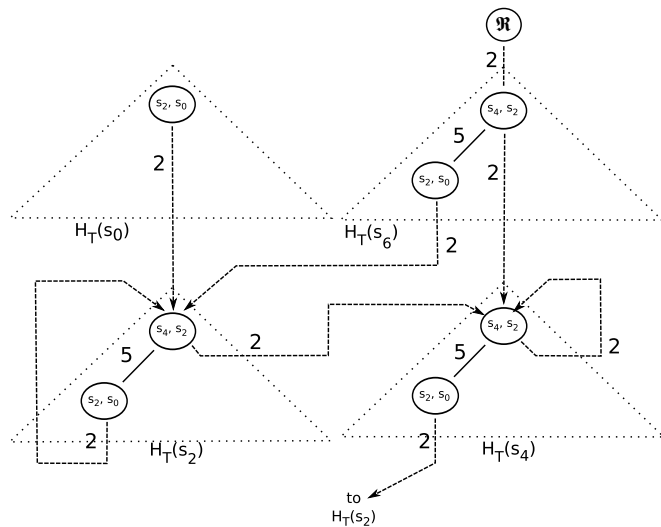
Figure 10: The path graph \mathcal{P}(G) (1) constructed by K^* at the point of A^* search presented in Figure 8, see the example in Section 4.6
