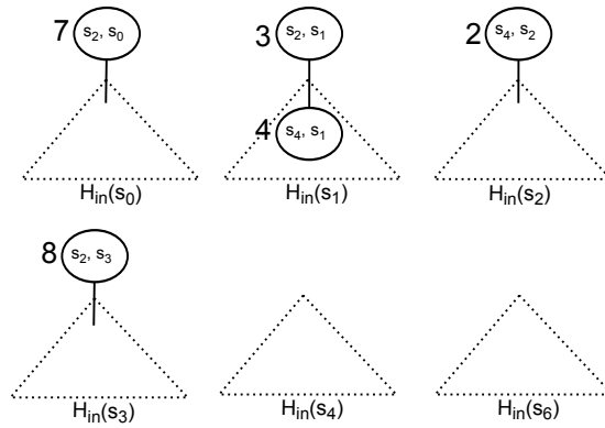
Figure 9: The H_{in} heaps constructed by K^* (1), see the example in Section 4.6
