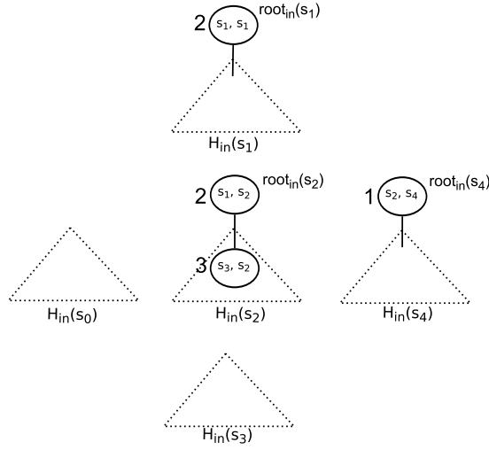
Figure 4: The incoming heaps H_{in}(\cdot) derived from the graph shown in Figure 3
