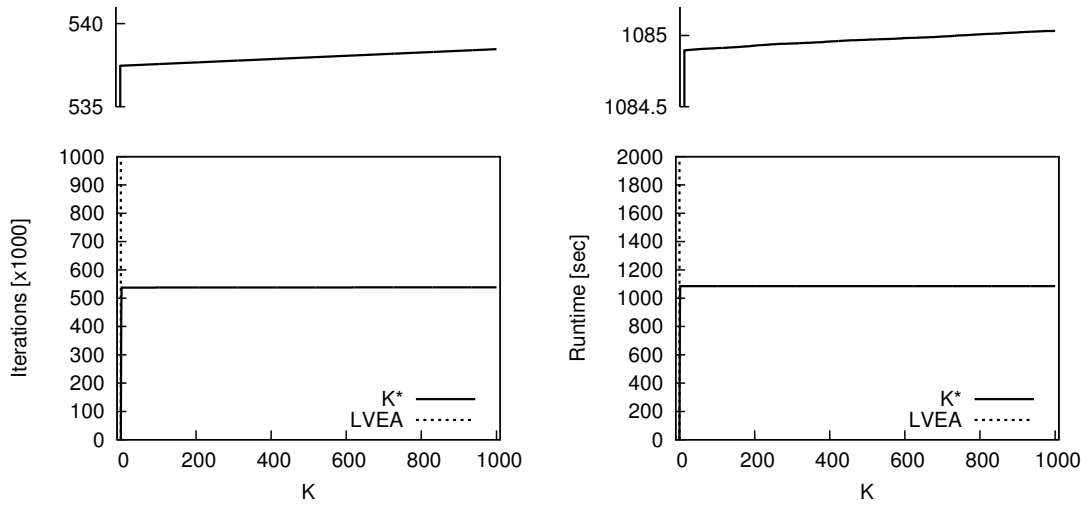
(a) Mean number of iterations needed for finding the routes. The diagram on the top zooms into the interesting segment of the curve of K^* .
