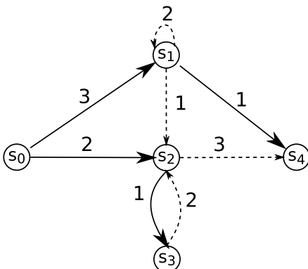
Figure 3: The same graph from Figure 2, where solid edges here represent the search tree as computed by A*. The dashed edges are the sidetrack edges.
