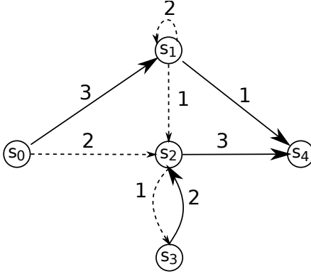
Figure 2: Example Graph, where the solid edges in the graph represent a reversed shortest path tree as computed by Eppstein’s algorithm (EA). The dashed edges are the sidetrack edges.
