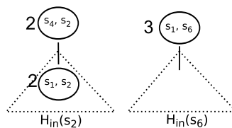
Figure 12: The modified H_{in} heaps after the extension, see the example in Section 4.6
