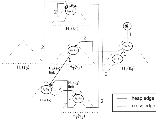
Figure 6: The path graph \mathcal{P}(G) computed by K^* from the graph shown in Figure 3
