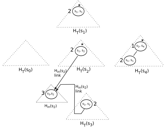
Figure 5: The tree heaps H_T(\cdot) derived from the graph shown in Figure 3
