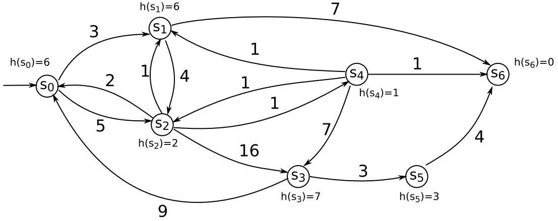
Figure 7: The problem graph G which is considered in the example explained in Section 4.6
