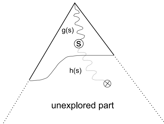
Figure 1: Illustration of A* search. The evaluation function f(s) = g(s) + h(s) determines the expansion order of vertices.
