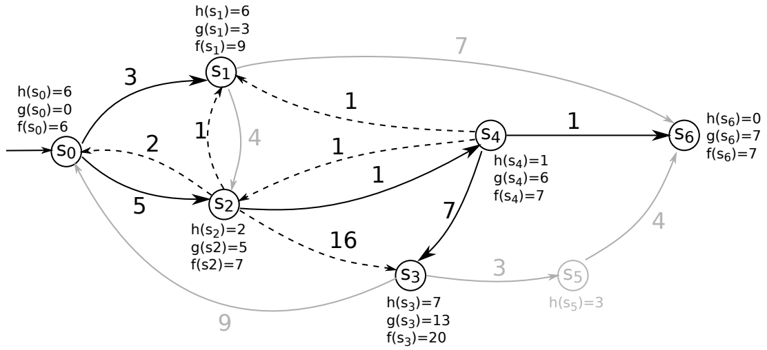
Figure 8: The explored part of G (1), see the example in Section 4.6. The faintly gray vertices and edges have not yet been explored by A^* . The solid line edges highlight the current search tree of A^* , whereas dashed line edges are the sidetrack edges.
