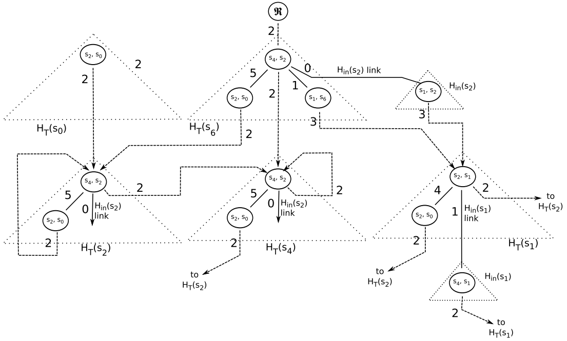
Figure 13: The path graph \mathcal{P}(G) (2) after the extension presented in Figure 11, see the example in Section 4.6
