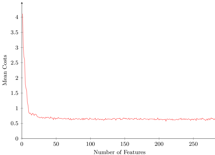
Fig. 2: Curve of the mean costs evaluated using a confidence threshold of 95% and 10-fold cross-validation with a fixed seed.
