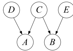
Figure 1. A common cause structure that gives rise to spurious regularities.
